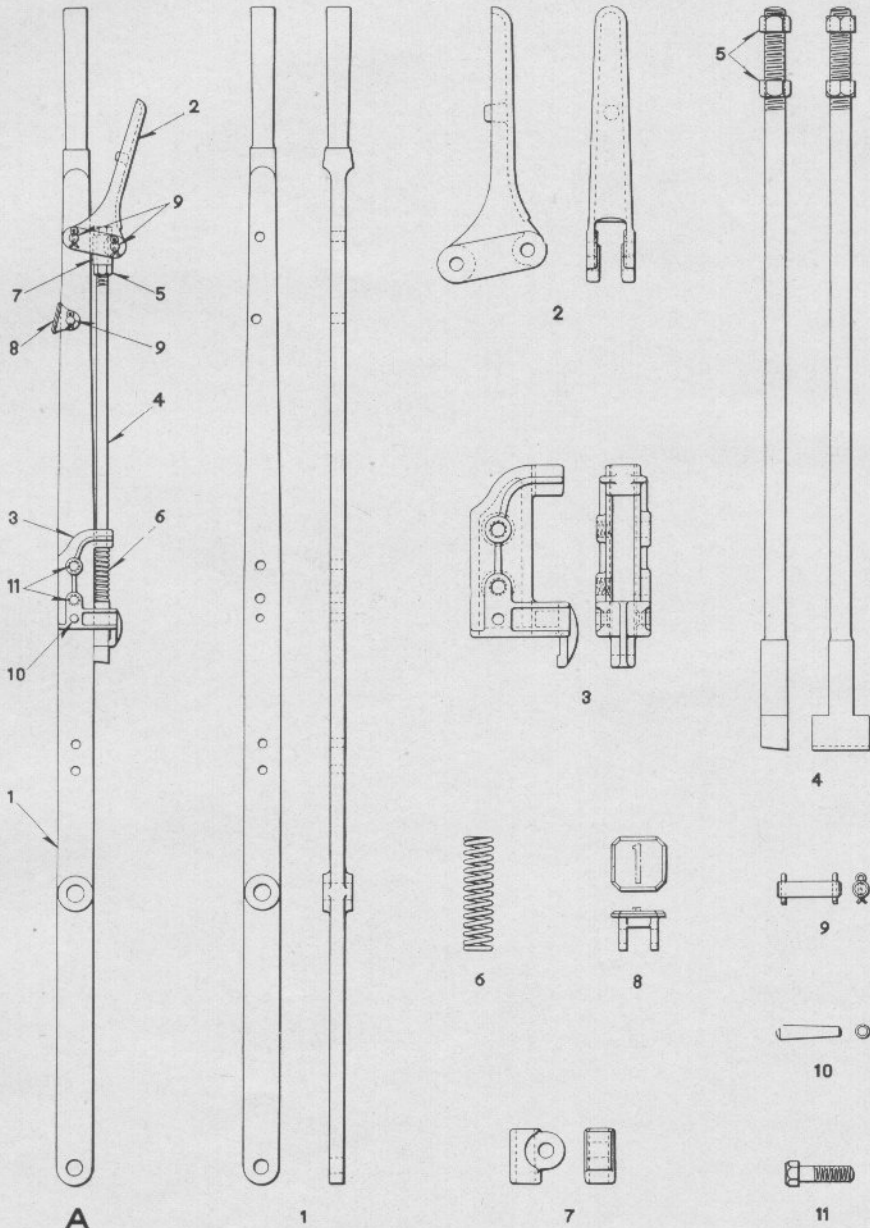
LEVER AND DETAILS FOR DWARF INTERLOCKING MACHINES
